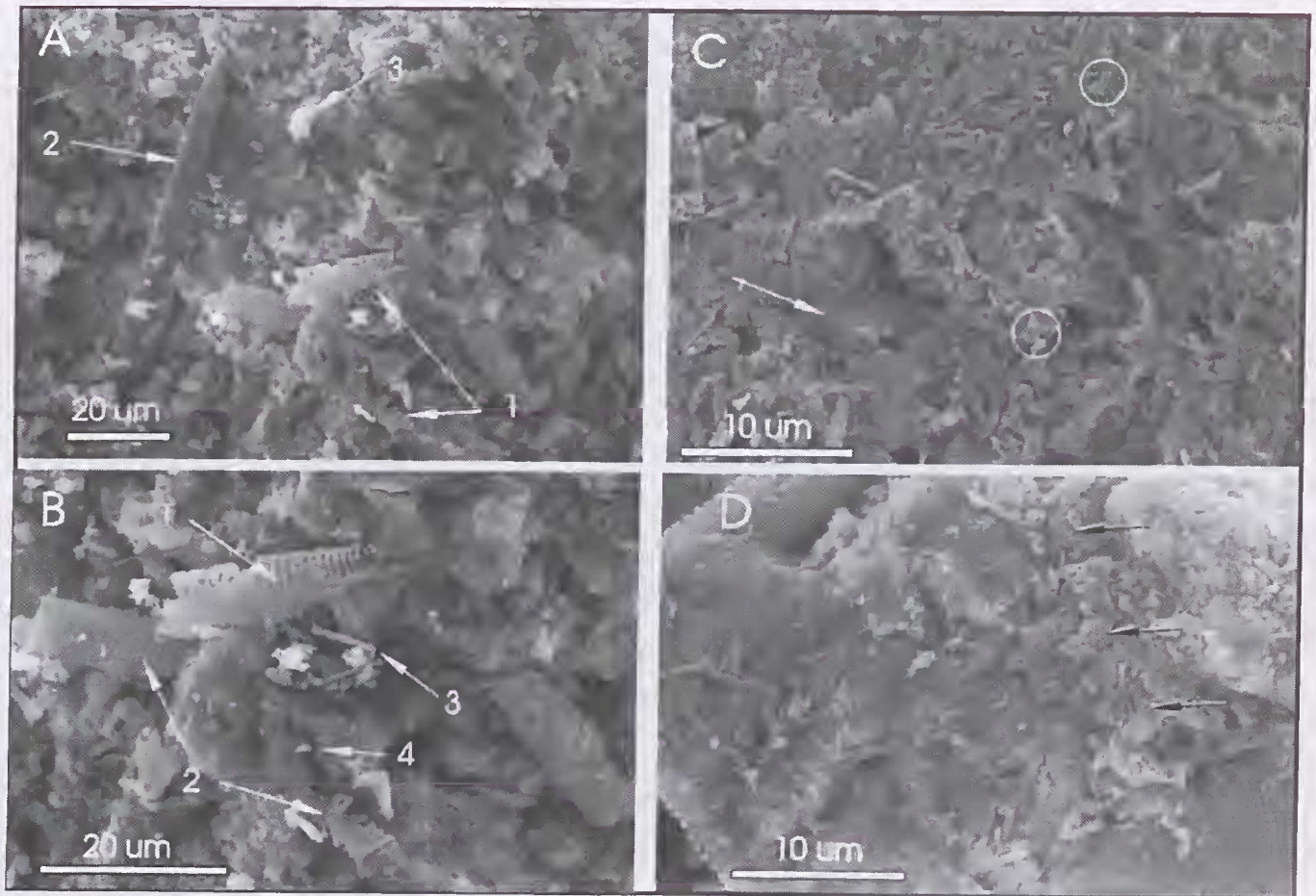
Figure 10. SEM photomicrographs of diatomite. A. Diatomite from a wetland basin in the Bassendean Dunes, east of Yanchep, showing typical view of diatom frustules in various stages of fragmentation (arrow 1), sponge spicule (arrow 2), and scattered kaolinite particles (arrow 3). B. Close-up showing the stages of fragmentation of diatom frustules: semi-complete diatom valve (arrow 1), 30 µm in size, fragmented valves (arrow 2) and (arrow 3), 15 µm in size, and 3–5 µm in size, respectively, leading finally to small fragments (arrow 4), < 1 µm in size. C. Close-up of diatomite from Lake Gnangara, showing diatoms in generally fragmented state; fragments show clear wall features such as sieve structure; particle sizes are mainly 1–5 µm; examples of diatom fragments < 1 µm in size are circled; the sample contains scattered quartz silt (arrow). D. Close-up of diatomite from Lake Gnangara showing diatom frustules in various stages of fragmentation from 3 µm in size, and showing wall structure (arrows), to 1–2 µm in size, and showing remnants of wall structure, to < 1 µm in size and structureless; the particles in this SEM view are adhering to a quartz silt particle (partial margin outlined).
